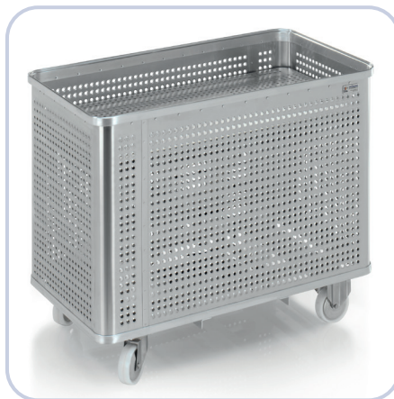
Cops trolley with spring-loaded base D04
